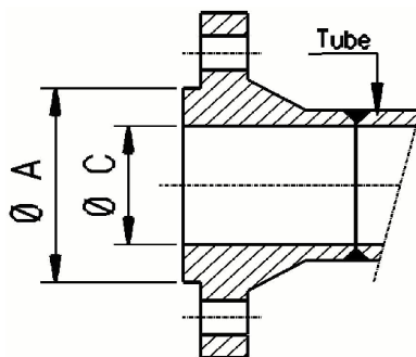
FLANGE TYPE 11
